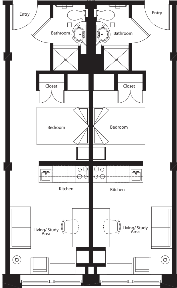
Typical Dorm Room Plan
